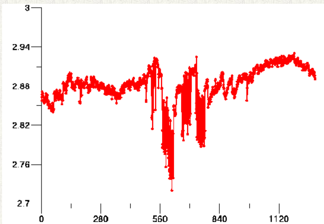
Magnetometer Plot of Solar Storm of Oct 24 2003
