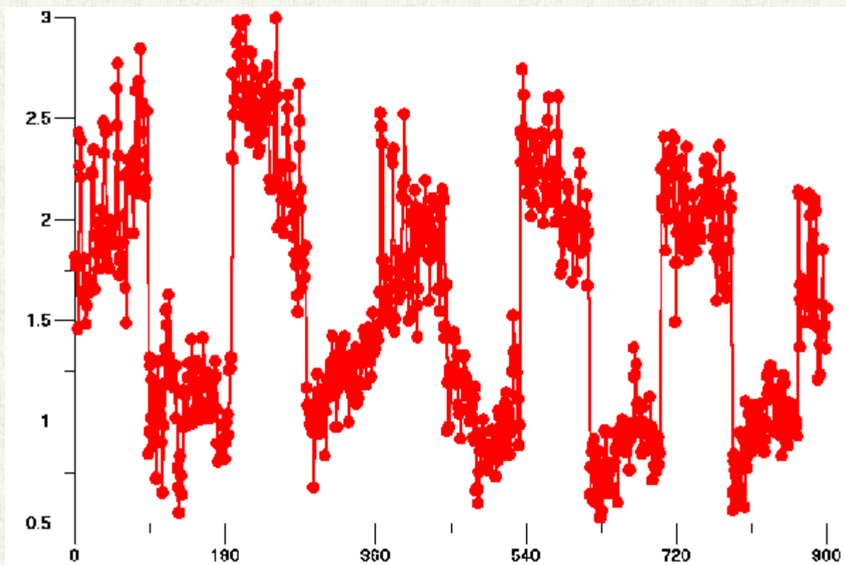
VLF Pulse Data Logged 040503 at approx. 1207-1225 X Axis : Observation No. (1 per second)
